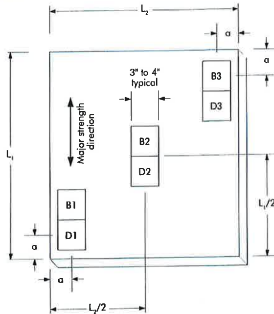
FIGURE 1 BLOCK SHEAR ("B") AND DELAMINATION ("D") SPECIMEN LOCATIONS \alpha = 4 \pm 1 inches, L_1 = 24 to 36 inches, and L_2 = 24 to 36 inches (1 inch = 25.4 mm)
